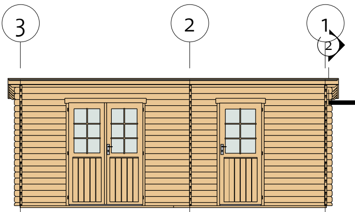
Roof 2
