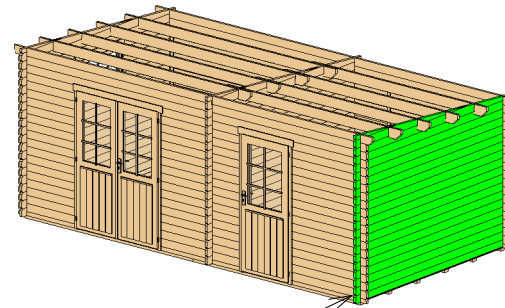
Wall 1
