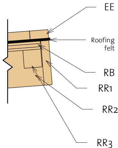
2 Roof reinforcement 1
